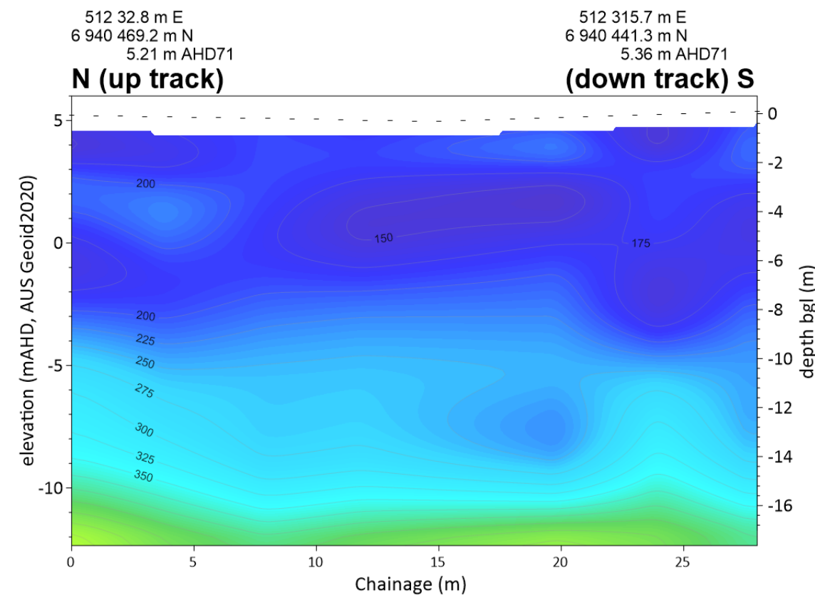
Seismic Line MASW AU-GP 148
